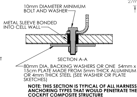
ANTI-SUBMARINE BELT MOUNTING
