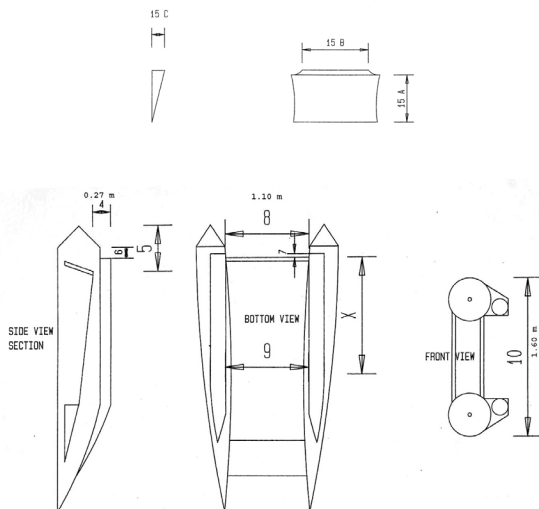
HULL DIAGRAM B:
