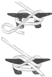
Half hitch
