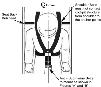
Figure "B" Anti-Submarine Belt
