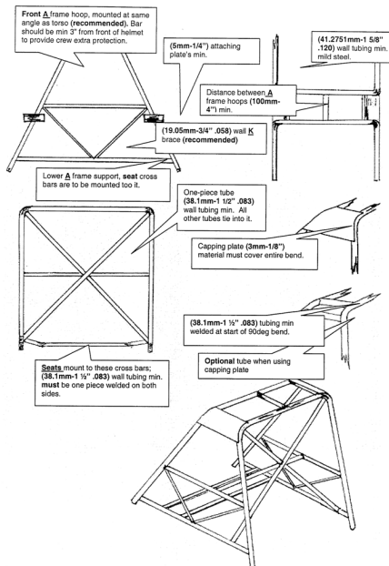
HELMET CLEARANCE
