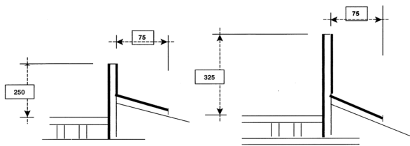
Sections B
