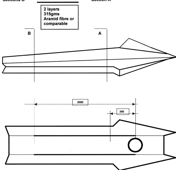
Sections B
