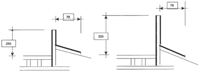
Sections B
