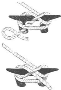
Half hitch
