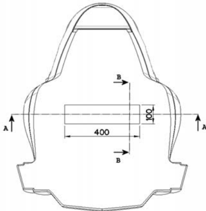
BACK VIEW OF THE SEAT-BACK BULKHEAD
